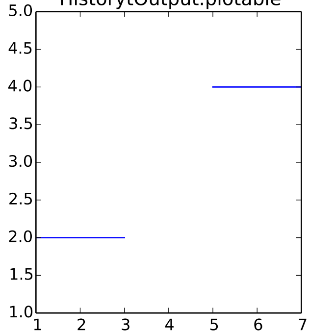
HistoryOutput.plotable
